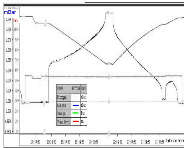
Figure 6: Radiator filling-purging cycle.
