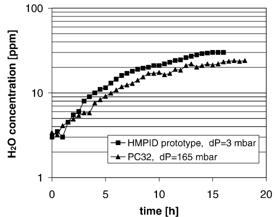
Fig. 2. Outgassed \text{H}_2\text{O} versus time.
