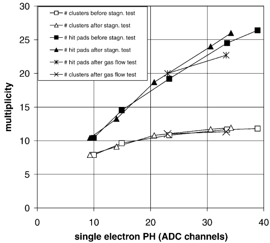
Fig. 4. Single-electron average PH versus multiplicity before and after the tests.
