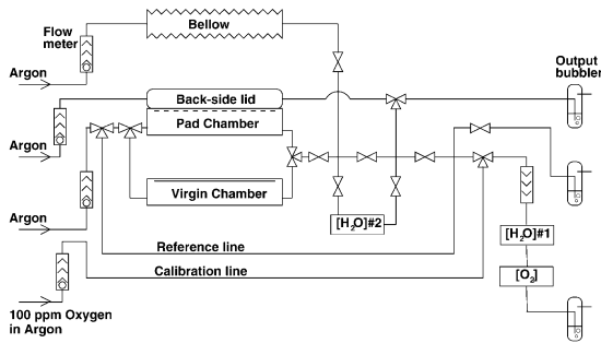
Fig. 1. The CsI PC outgassing test setup.
