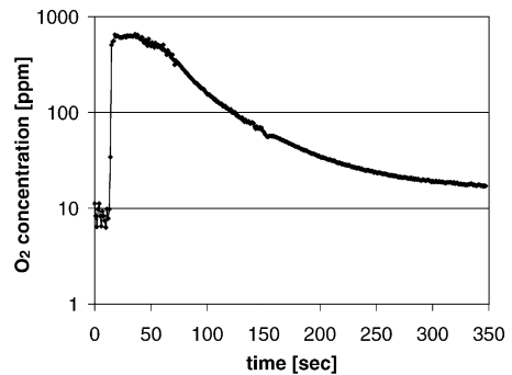
Fig. 3. PC24, output \text{O}_2 concentration after 2 h stagnancy.
