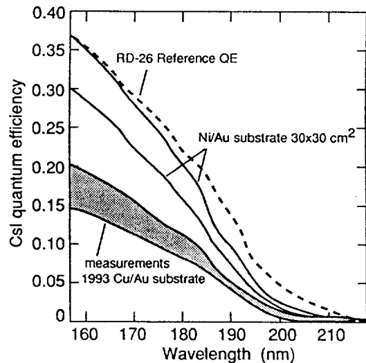
Fig. 2. The CsI QE reference curve (dotted line) compared to QE curves used to fit experimental data. The two upper curves delimit the QE measured on five CsI PCs using the new Ni/Au substrates. The hatched area corresponds to PCs using the old substrates.
