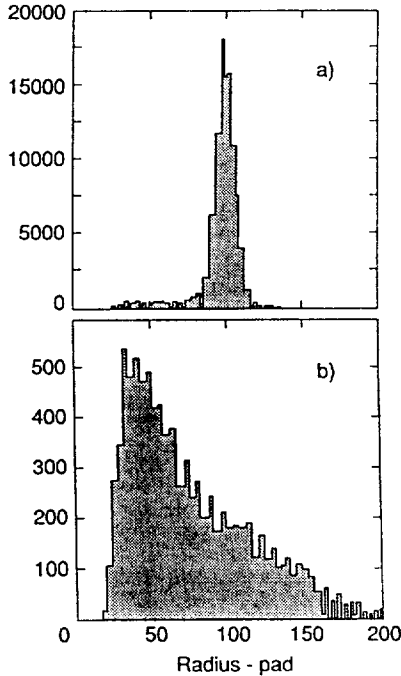
Fig. 3. Radial distributions of pad hits in methane: (a) with a 10 mm C 6 F 14 radiator and a 3 mm quartz plate, illustrating the small background relative to the Cherenkov peak; (b) only with the quartz plate, illustrating the shape of the emitting background source (avalanche and quartz).
