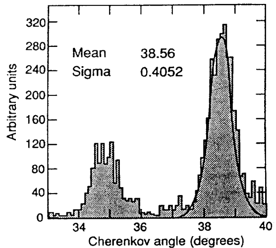
Fig. 4. Results of the analysis of high-density events (50 part./m 2 ) using randomly superimposed experimental events obtained with π/p 70:30 of 3 GeV/c momentum.
