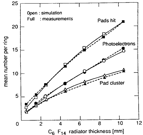
Fig. 1. Results of the CsI-fast RICH using the G10/Cu/Ni/Au pad electrode with 3 \text{ GeV}/c pions and ring radius of 98 mm as function of the radiator thickness.
